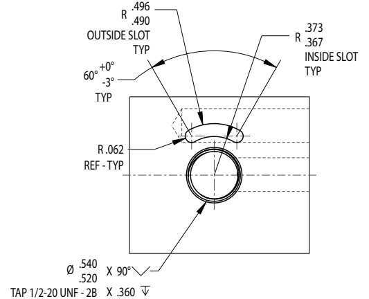
Manifold Valve/ Manifold Interface
