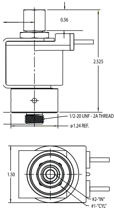
3-Way Line Connect 2-Way Normally Open Manifold Mount
